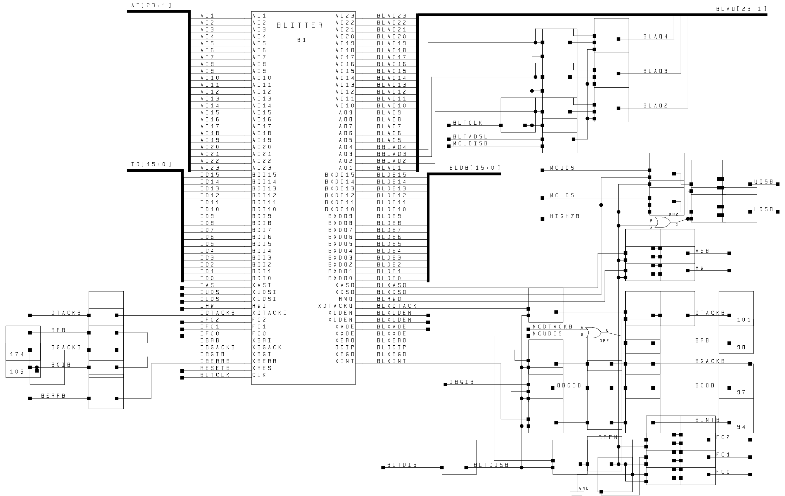
COMBEL - Top Level: BLITTER
